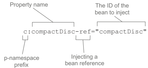
Figure 2.2 Injecting a bean reference into a property with Spring's p-namespace
