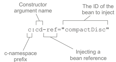
Figure 2.1 Injecting a bean reference into a constructor argument with Spring's c -namespace
