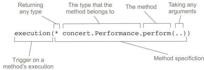
Figure 4.4 Selecting Performance 's perform() method with an AspectJ pointcut expression
